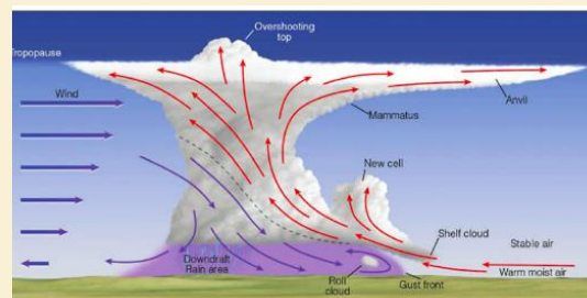
ctive FIGURE 10.5 A simplified model describing air motions and other features associated with an intense multi-cell thunderstorm that has a tilted updraft. The severity depends on the intensity of the storm's circulation pattern.
